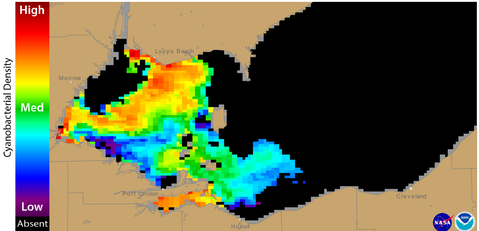
Figure 1. Cyanobacterial Index from NASA MODIS-Terra data collected 24 September, 2017 at 11:55 EST. Grey indicates clouds or missing data. The estimated threshold for cyanobacteria detection is 20,000 cells/mL.
