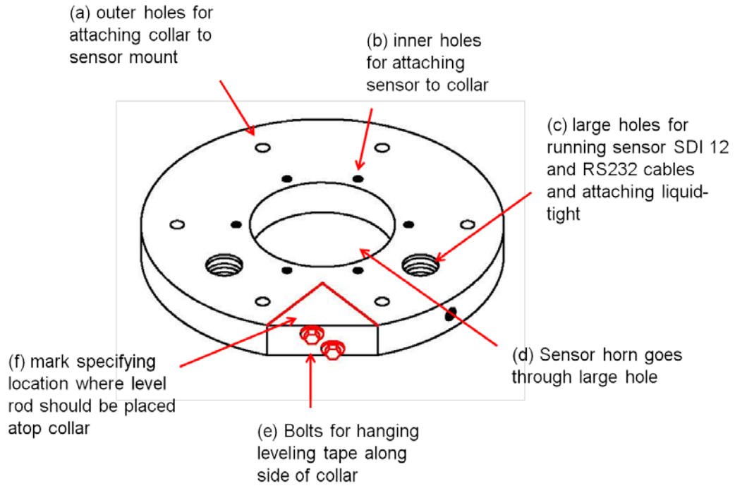
Figure 3-5. Annotated schematic of the WaterLog ® sensor's leveling collar.
