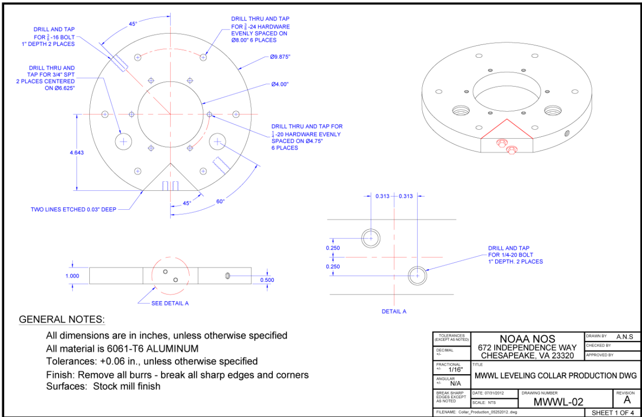
Figure 3-4. Engineering drawing of microwave radar sensor leveling collar.
