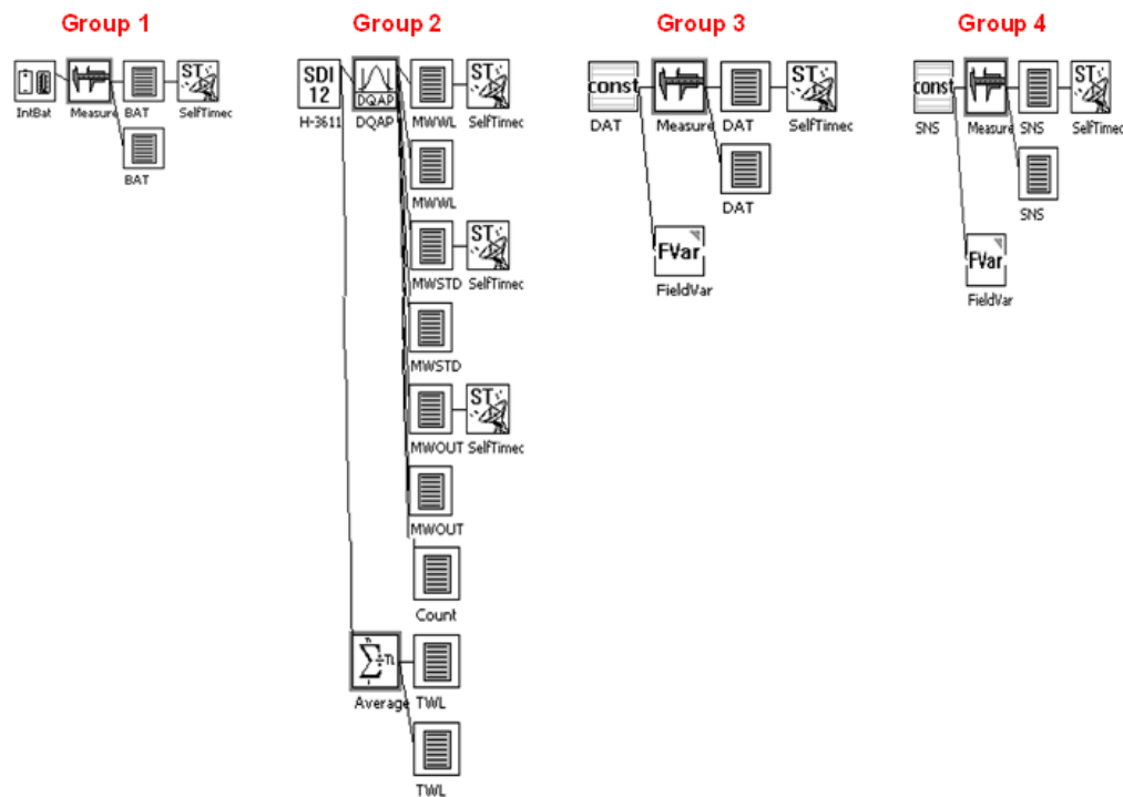
Figure 3-28. Final graphical setup for a WaterLog ® sensor, which is configured by CIL/SIL prior to deployment.
