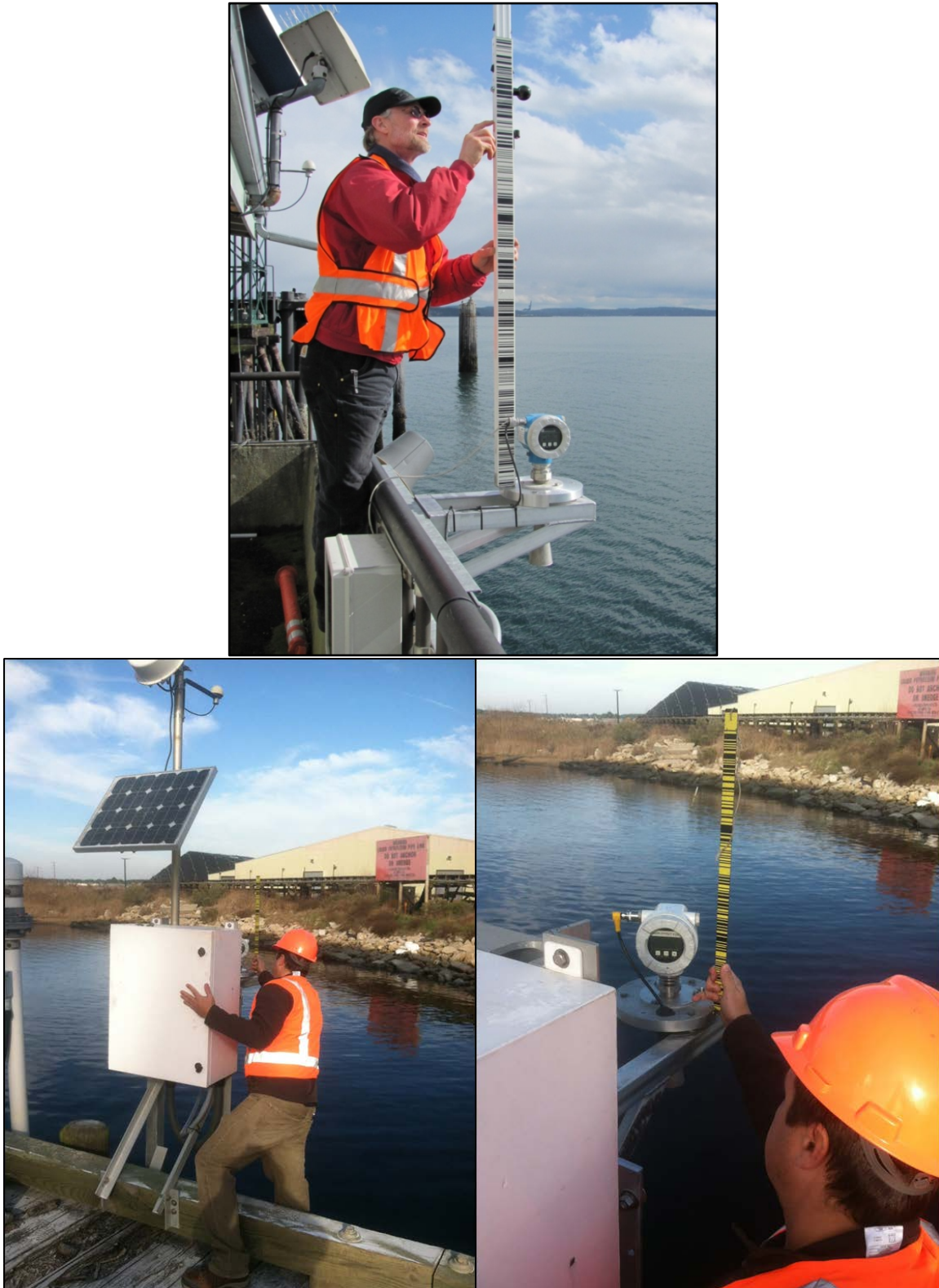
Figure 3-9. Examples of geodetic level conducted with leveling point atop the collar surface.
