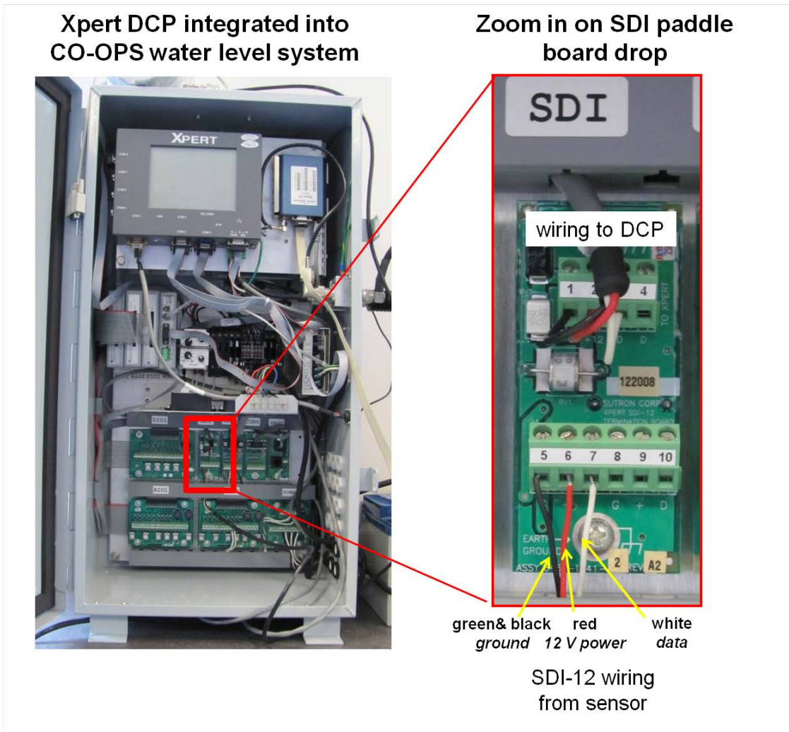
Figure 3-16. SDI-12 terminal board (paddle board) dropped from DCP's SDI 12 panel in typical CO-OPS system.
