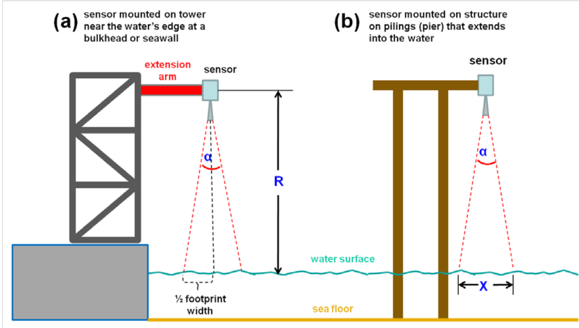
Figure 3-10. Depiction of two different types of installation scenarios; (a) sensor mounted on a structure at the water’s edge and (b) sensor installed on a structure on pilings that extend out into a body of water.
