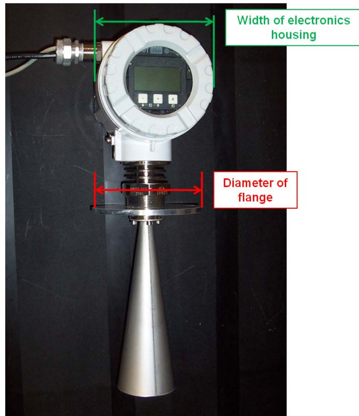
Figure 3-3. Width of sensor body is larger than diameter of sensor flange, so a level rod could not be set atop the flange.
