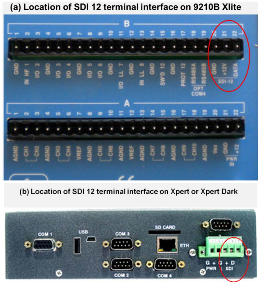
Figure 3-15. SDI-12 term board for (a) 9210B Xlite and (b) Xpert and Xpert Dark.
