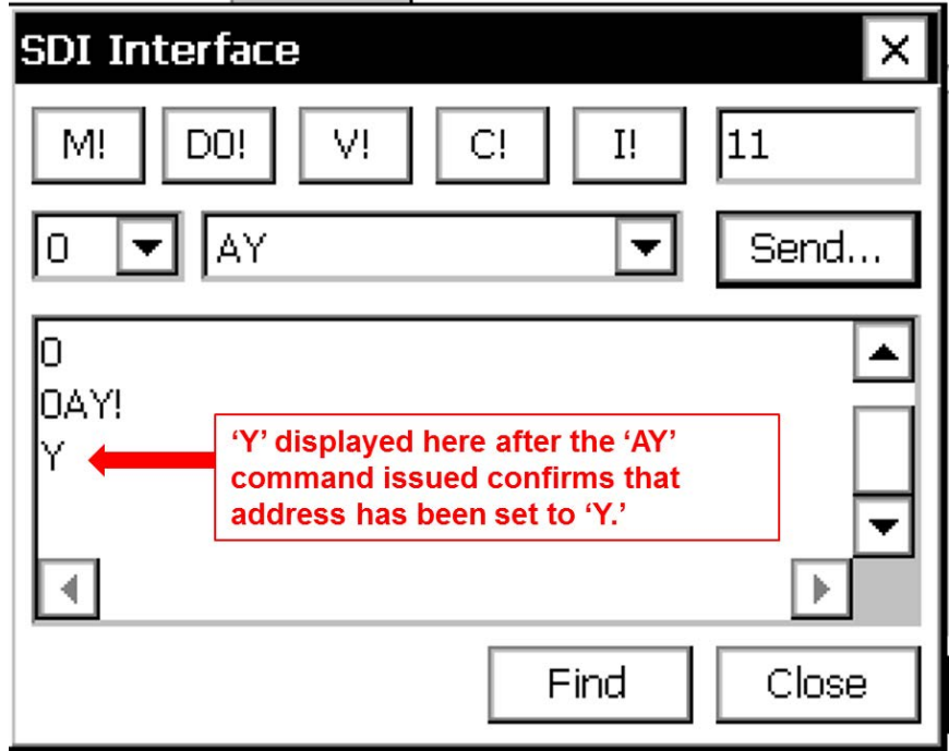
Figure 3-23. Value 'Y' displayed after AY command issued.
