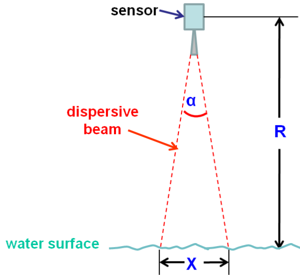
Figure 3-1. Depiction of radar’s dispersive beam with labels representing variables in (1).
