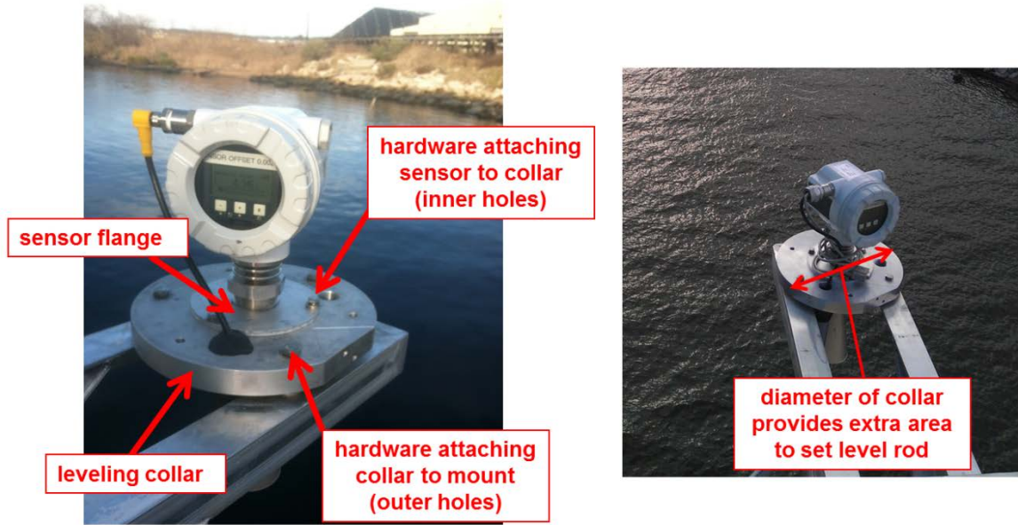
Figure 3-7. Examples of field installations showing WaterLog ® sensor mounted in leveling collar.
